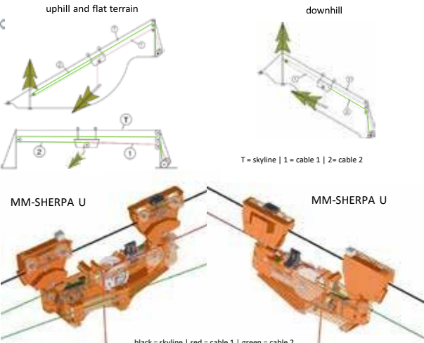
MM-SHERPA U® 3-cable system (uphill, flat terrain & downhill) 3to / 4to
